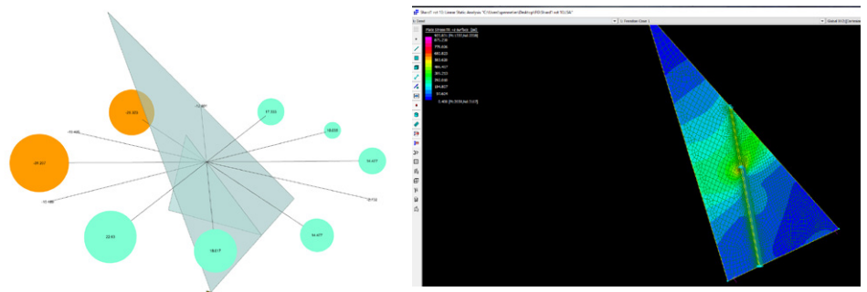
Figure 2: Left: Grasshopper Script Toolbox. Right: Strand7 Finite Element Analysis.
