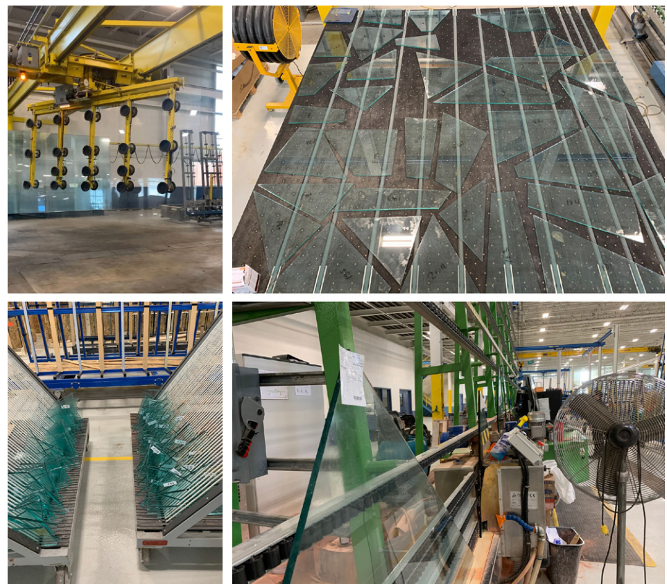
Figure 4: Glass Fabrication by Agnora.
